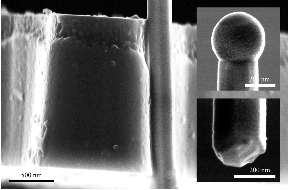
Figure 4.7. | SEM images showing parts of the CoFeB nanotube C2. In the main frame we see C2 affixed to an ultrasoft cantilever in configuration [2], facing the tip of the cantilever, and in the two insets, the two ends of C2 are depicted.
