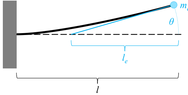
Figure 3.1. | Illustration of a mechanical oscillator in cantilever configuration. Definition of the effective length l_e compared to cantilever length l . Illustration not to scale.
