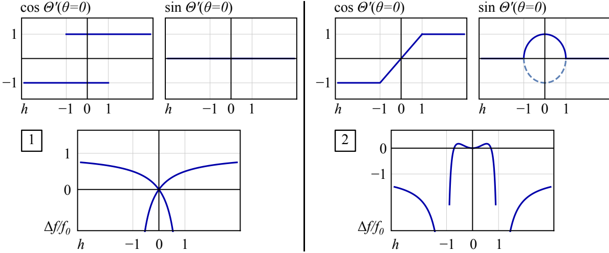
Figure 3.4. | Graphs of the torque-reduced relative frequency shift \Delta f/f_0 vs. the reduced applied field h from equations (3.19) for configurations [1] and [2]. Dashed lines are horizontal and vertical asymptotes.
