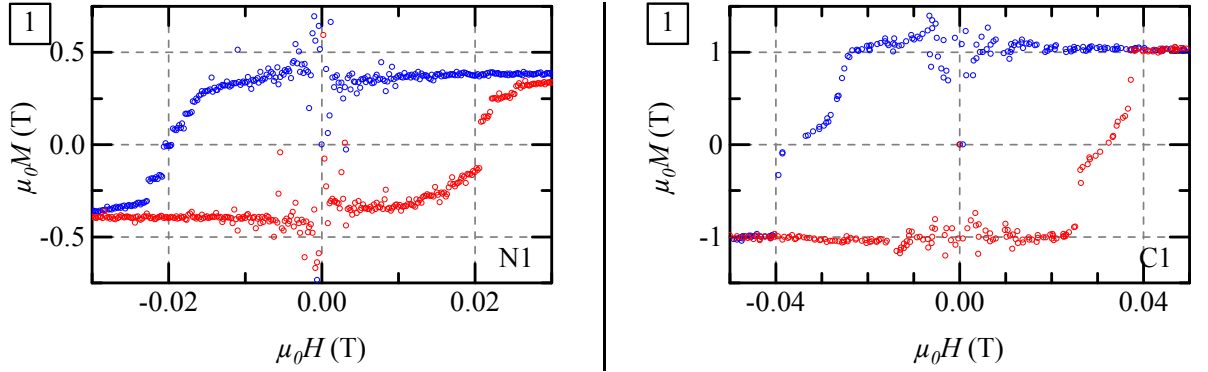
Figure 5.5. | Graphs of the magnetization \mu_0 M as a function of the applied field \mu_0 H (both in units of T) for configuration [1] of the Ni sample N1 (left hand side) and the CoFeB sample C1 (right hand side).
