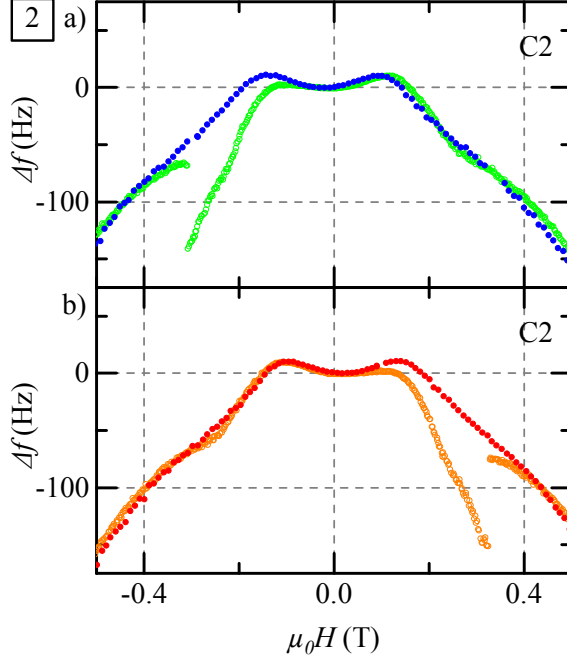
Figure 5.8. | DCM measurements of sample C2 in configuration [2]. The frequency shift \Delta f is plotted as a function of the applied field \mu_0 H . The graph compares jump- (green, orange) and no-jump-case (blue, red) in negative (a), and positive (b) applied field sweep direction, respectively, at low applied field range.
