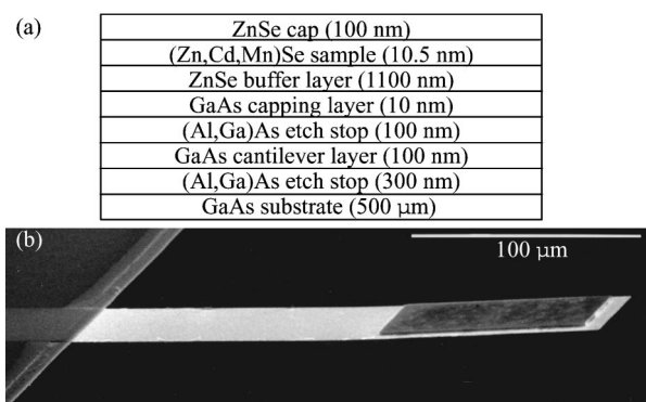
FIG. 1. (a) Schematic of the MBE-grown heterostructure. The 10.5-nm-thick magnetic layer is grown as a digital alloy (seven iterations of: 1/16th monolayer of MnSe followed by 4 15/16th monolayer of Zn_{0.87}Cd_{0.13}Se ). The etch stop layers are grown as a random alloy ( Al_{0.7}Ga_{0.3}As ). (b) SEM photo of a 100-nm-thick, 250\ \mu m long cantilever supporting a rectangular mesa of paramagnetic (Zn,Cd,Mn)Se .
