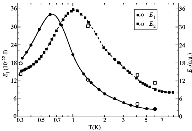
FIG. 3. \Delta E_1 and \Delta E_2 as a function of temperature at H=2 T. Each data point is acquired with the temperature of the cryostat held constant. Solid symbols are measurements of the drive amplitude required to maintain constant cantilever amplitude; hollow symbols are from fits of the cantilever resonance curve. The lines are guides for the eye.
