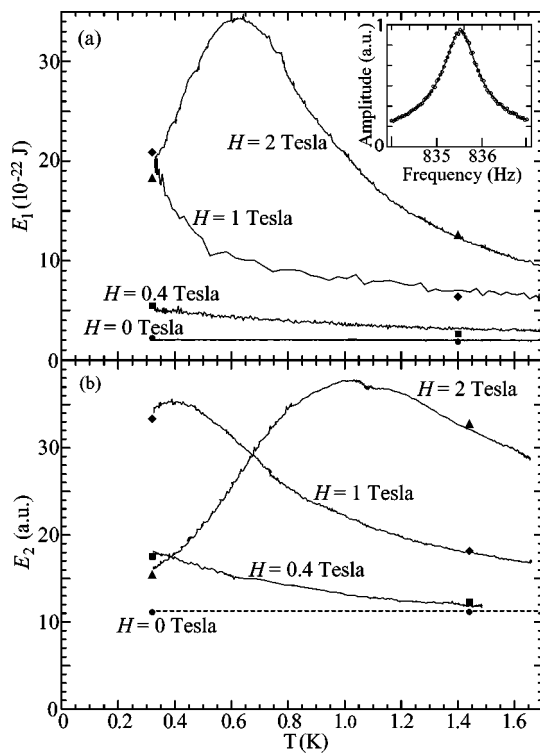
FIG. 2. (a) \Delta E_1 as a function of temperature for various values of the applied magnetic field. Inset: resonance curve of the lever at T=0.32 K, B=2 T (open points) and fit to a damped simple harmonic oscillator (solid line). (b) \Delta E_2 as a function of temperature for various values of the applied magnetic field. In both plots the solid lines are taken as the temperature of the cryostat is slowly changed. The solid points ( \bullet H=0 T; \blacksquare H=0.4 T; \blacklozenge H=1 T; \blacktriangle H=2 T) are from fits of the cantilever resonance taken at fixed temperature. The dashed line in (b) is a guide for the eye.
