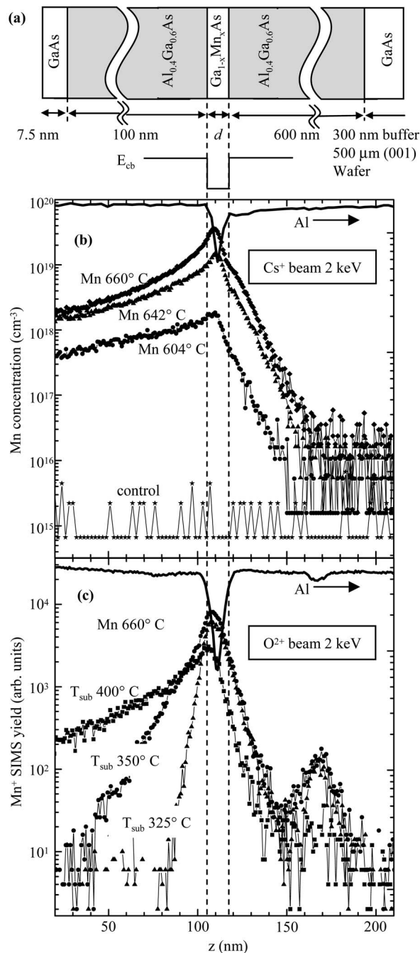
FIG. 1. (a) Schematic of sample layer structure and conduction-band energy along the growth axis z . (b) Mn concentration profile measured by SIMS for four 7.5-nm QWs with varying Mn-doping level (Mn effusion cell temperatures marked in the figure) and (c) for QWs with the same Mn-doping level but varying substrate temperatures (marked in the figure). The uncalibrated Al SIMS signal (plotted as black lines) serves as a marker for the QW region.
