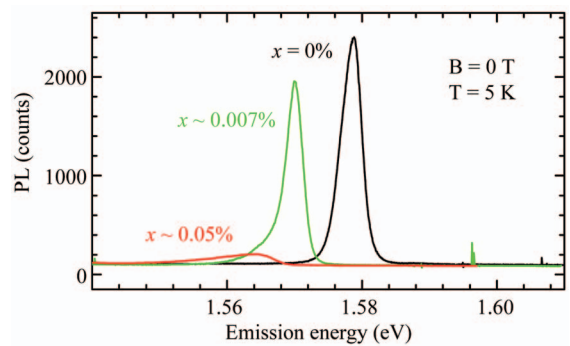
FIG. 16. (Color) PL plotted as a function of emission energy for a set of 7.5-nm QWs with varying Mn doping; the samples are excited with 1 \text{ W/cm}^2 at 1.722 \text{ eV} . Samples with x > 0.13\% showed no PL.
