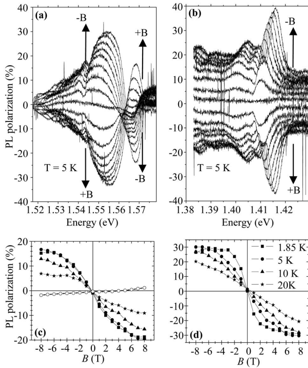
FIG. 19. PL polarization spectra for a 7.5-nm GaMnAs QW with an 1.72-eV excitation at 1.0 mW (a) near the QW emission peaks ( \sim 1.6 eV) and (b) at the bulk Mn-acceptor line for GaMnAs ( \sim 1.4 eV), which results from unintentional Mn doping in the 300-nm-thick GaAs buffer layer. The spectra are plotted as a function of emission energy for different magnetic fields from -8 to +8 T at 1-T intervals. (c) The PL polarization integrated over a single emission peak as a function of B for the high-energy ( \sim 1.57 eV at T=5 K, open circles) and low-energy ( \sim 1.55 eV at several temperatures, solid symbols) peaks and (d) for the bulk Mn-acceptor line peak plotted for several temperatures.
