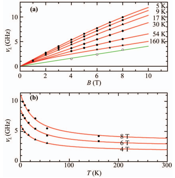
FIG. 10. (Color) Temperature dependence of \nu_L for 7.5-nm quantum wells. (a) The effect of increasing T on the B dependence of \nu_L for the sample with x \sim 0.007\% (solid points) and for the x=0 sample (open points). (b) T dependence of \nu_L at constant B for the x \sim 0.007\% sample. Red lines in (a) and (b) are fits to Eq. (4).
